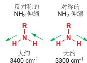
Interactive vibrations of methylamine
