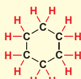
环 (ring)
