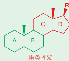
甾类骨架
