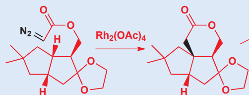
路线 1: Cane
